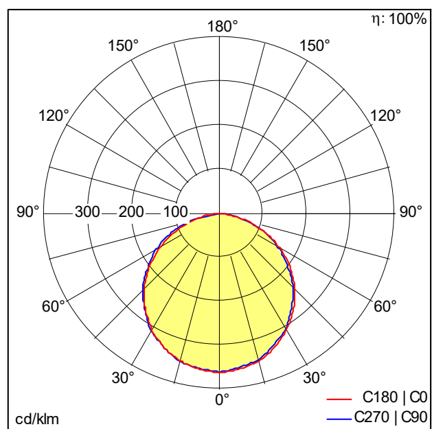
TE_ZOE_LED_DL_210_2000_830.ltd
