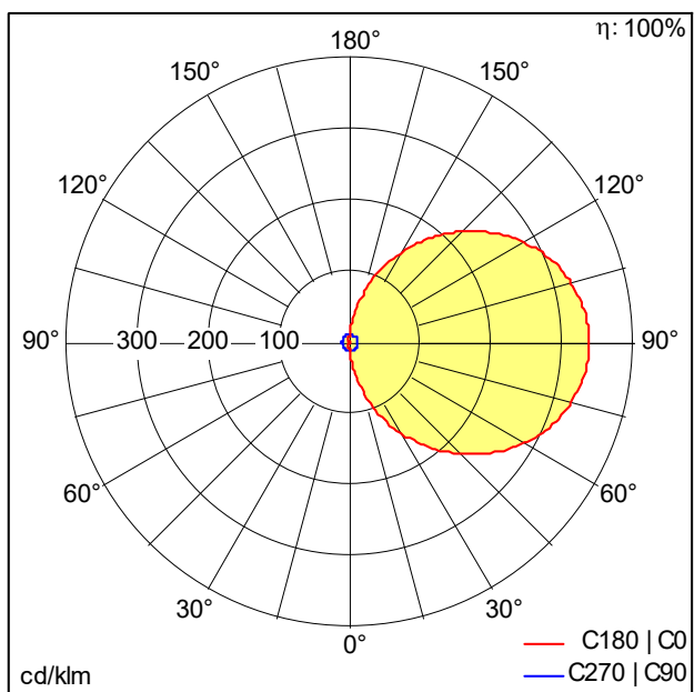
TE_LARA_LED_250_800_840_WH_E3e.ltd
