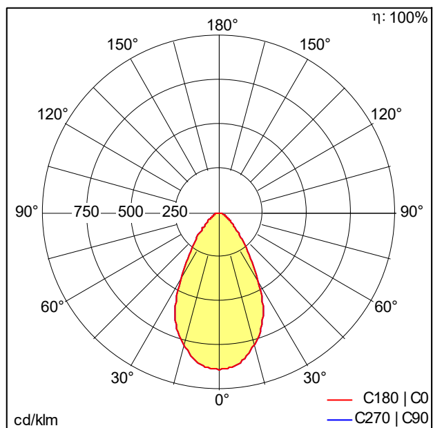
TE_GEORGE_LED_330_12000_840.ltd
