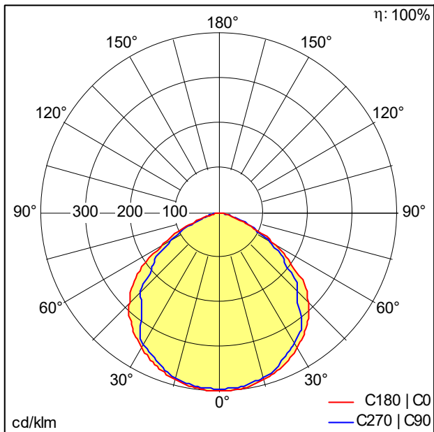
TE_LEONIE_LED_FL_IP65_50W_830.idt
