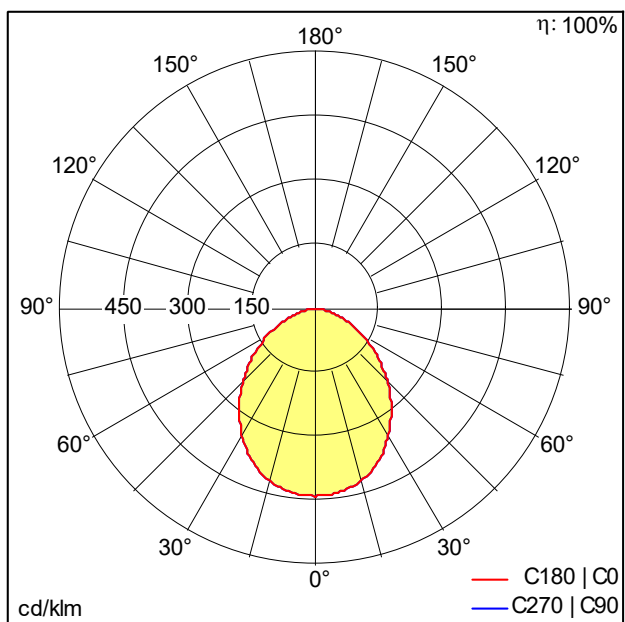
AMY_VARIO_200_LED_DL_2000_840.idt
